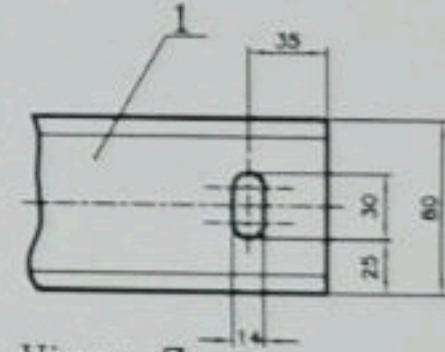
View: Z 1:2.5
