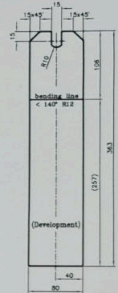
No. 2 1:2.5
